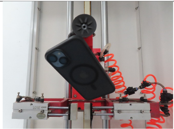
During test-Drop corner
